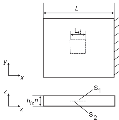
Figure 1: Geometrical representation of the plate.
