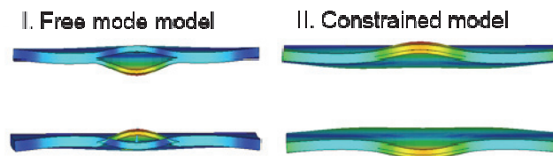
Figure 2: Models of delamination.
