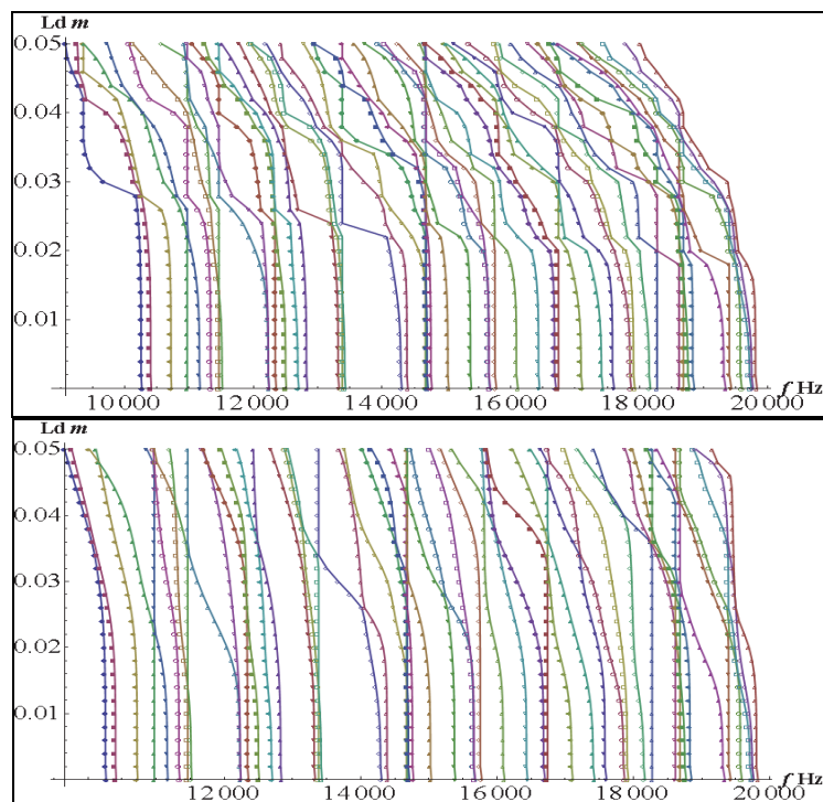
Figure 4: Shifts of natural frequencies in the range of 10-20 kHz.
