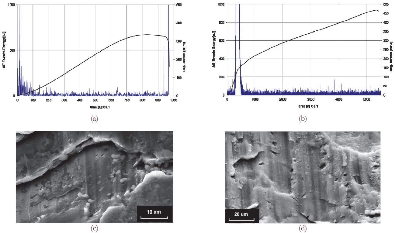
Figure 8: AE behavior and the course of external load: (a) up to all-out breaking and (b) exactly just before breaking of the Mg 4 Li 5 Al sample; (c) and (d) – corresponding SEM images.
